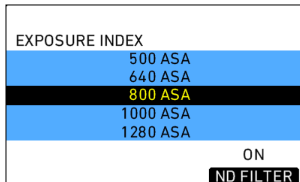
Figure 112: EI screen
