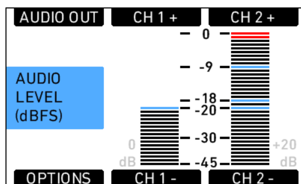
Figure 46: Audio screen
