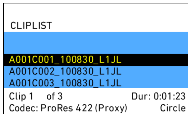
Figure 69: CLIPLIST screen
